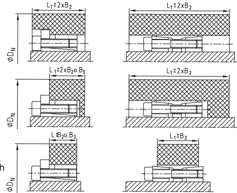
Mounting conditions of clamping set
